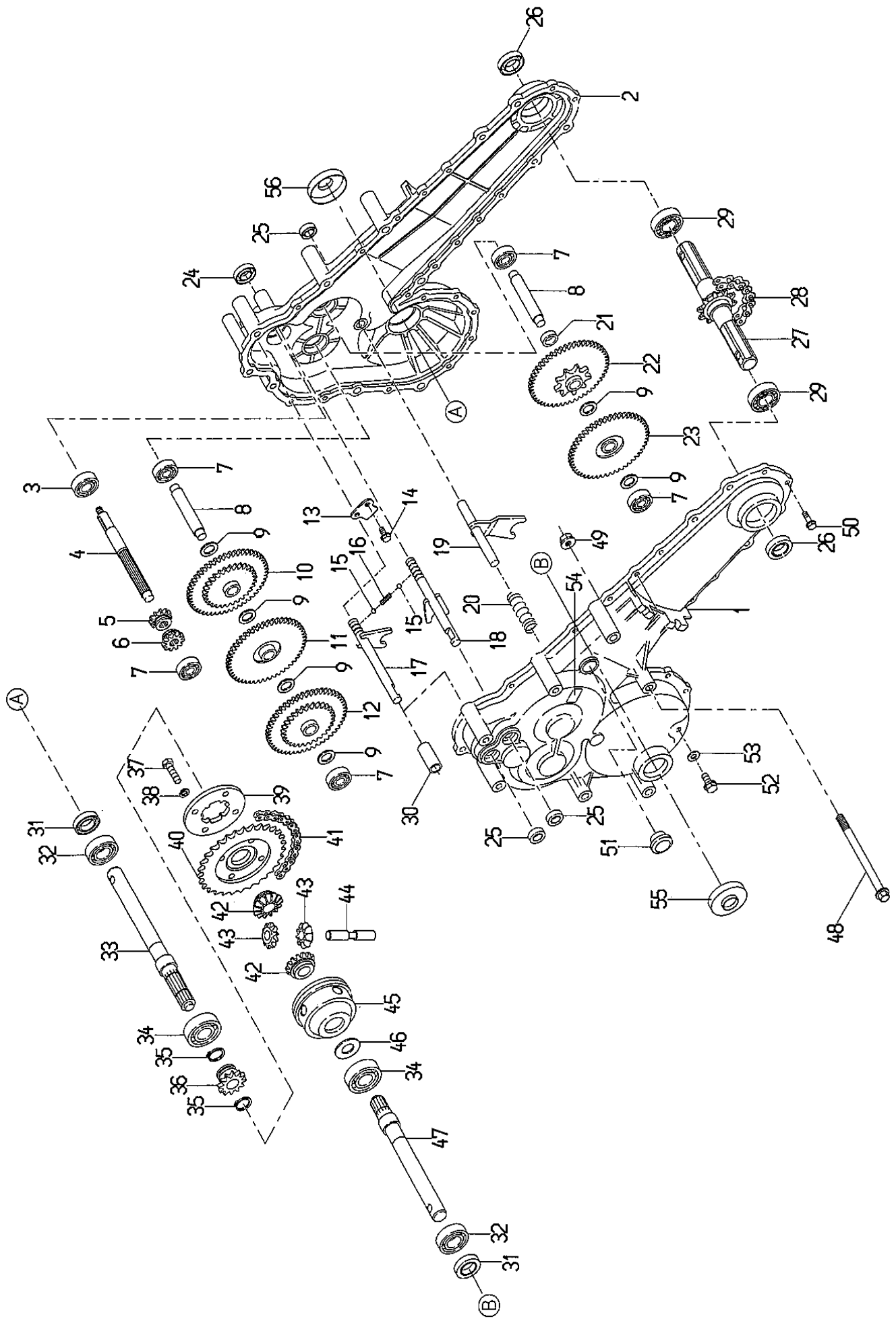
Fig. 2 TRANSMISSION
